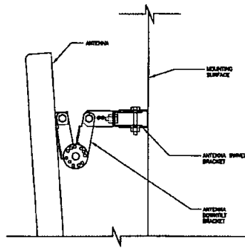
ANTENNA MOUNT 3"=1'-0"
