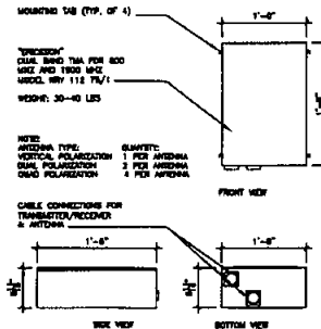
TMA UNIT 1'-1/2"=1'-0"
