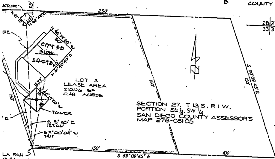
PLOT PLAN
