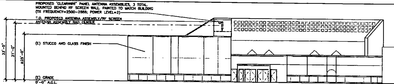
NORTH ELEVATION
