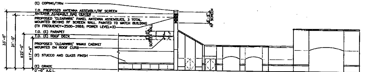
EAST ELEVATION
