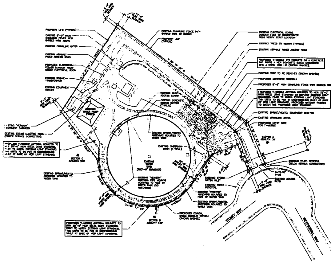
SITE PLAN SHEET 1 OF 1
