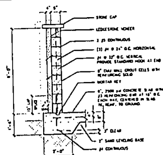
12 NEW CMU ENCLOSURE WALL SECTION SCALE: 1/4" = 1'-0"
