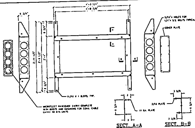
5 MICROFLECT 'BTS' BASE FRAME SCALE: 1/4" = 1'-0"
