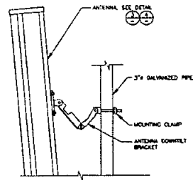
ANTENNA MOUNTING 1'-1/2" x 1'-0"
