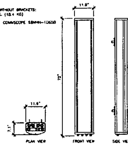
6' HEXPORT COMMSCOPE ANTENNA 3/4" x 1'-0"
