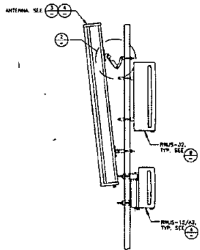
ANTENNA MOUNT 3/4" x 1'-0"
