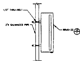
RRUS-32 MOUNTING 1" x 1'-0"
