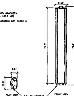
6' HEXPORT KATHREIN ANTENNA 3/4" x 1'-0"
