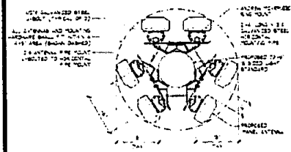
02 ANTENNA PLAN DETAIL SCALE: 3/4" = 1'-0"
