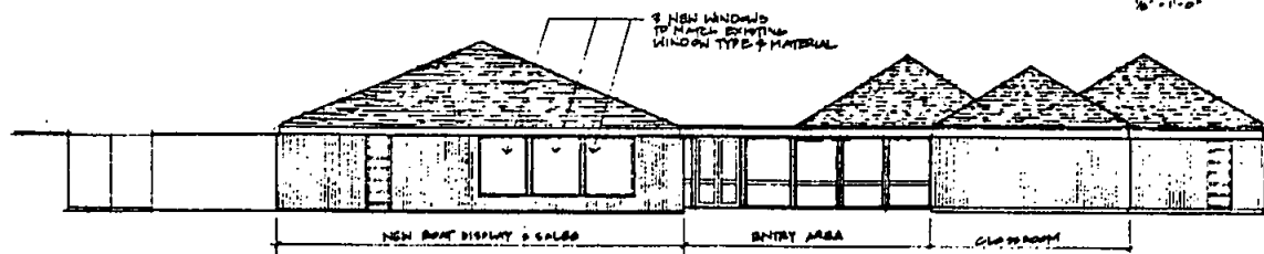
SOUTH ELEVATION 76' - 11-0"
