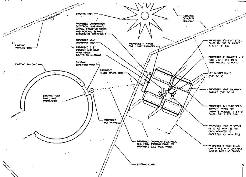
AREA PLAN 1/4" = 1'-0"
