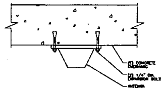
TYP DAS ANTENNA TO CONCRETE CEILING 3"=1'-0"
