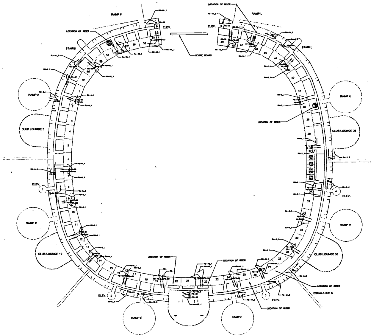
ANTENNA SCHEMATIC AT PRESS LEVEL 1"=40'
