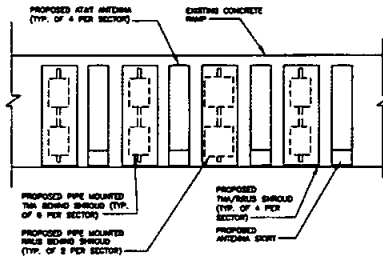
TYPICAL ELEVATION AT ANTENNAS 3/8"=1'-0"
