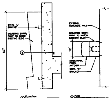
ANTENNA SKIRT 1"=1'-0"
