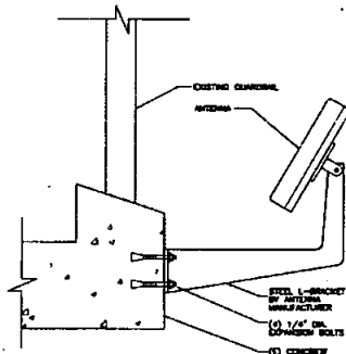
TYP. DAS ANTENNA AT INTERIOR GUARDRAIL NTS
