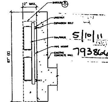
TMA/RRUS MOUNTING 1"=1'-0"
