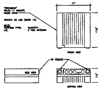
RRUS 1-1/2"=1'-0"
