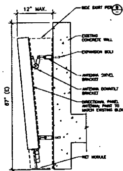
ANTENNA MOUNTING 1"=1'-0"
