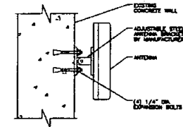
TYP DAS ANTENNA TO CONCRETE WALL 3"=1'-0"
