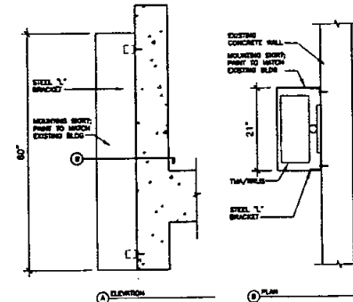
TMA/RRUS SHROUD 1"=1'-0"
