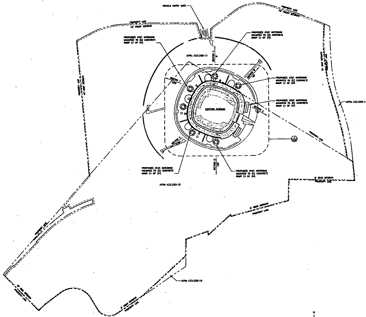
SITE PLAN 1"=200'
