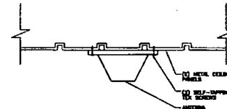
TYP DAS ANTENNA TO METAL PANEL CEILING 3"=1'-0"
