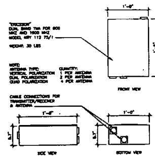
TMA UNIT 1-1/2"=1'-0"
