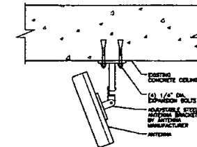
TYP DAS ANTENNA TO CONCRETE CEILING 3"=1'-0"
