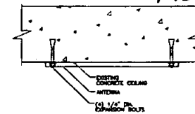
TYP DAS ANTENNA TO CONCRETE CEILING 3"=1'-0"
