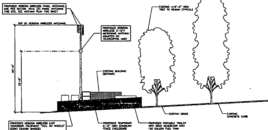
WEST ELEVATION
