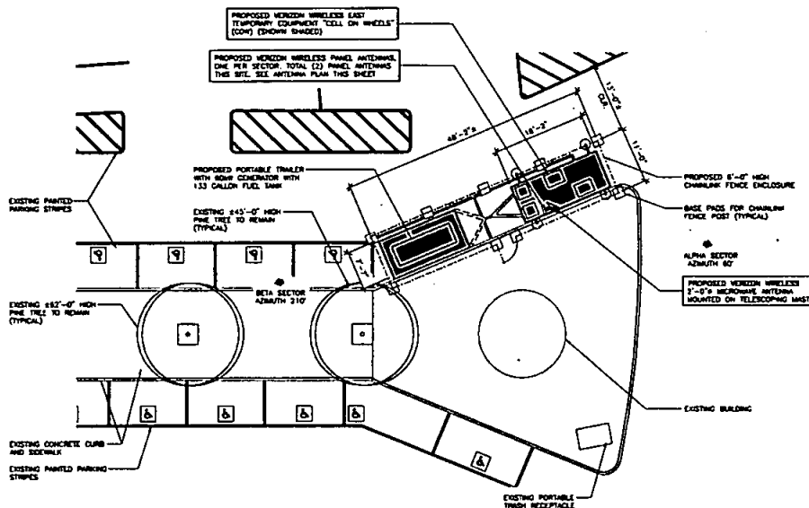
ENLARGED SITE PLAN (EAST)
