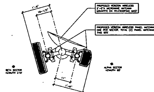
ANTENNA PLAN
