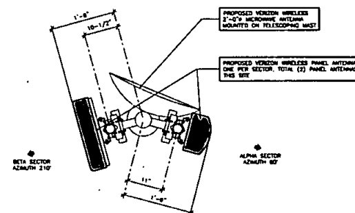
ANTENNA PLAN
