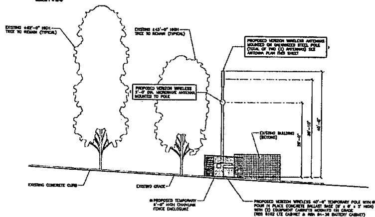
WEST ELEVATION
