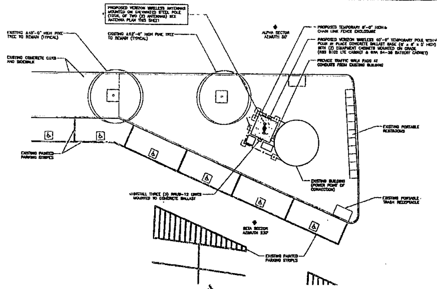
ENLARGED SITE PLAN SITE #4 SOUTHEAST
