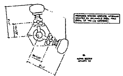
ANTENNA PLAN
