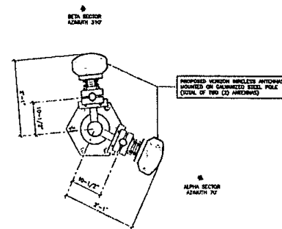
ANTENNA PLAN SCALE 1" = 10'-0"
