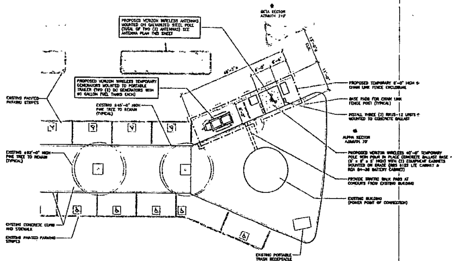
ENLARGED SITE PLAN SITE #1 NORTHEAST SCALE 1" = 10'-0"
