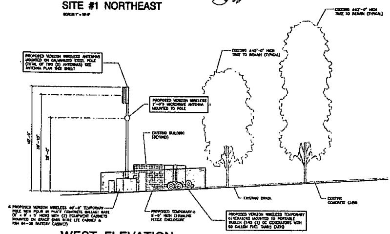
WEST ELEVATION SCALE 1" = 10'
