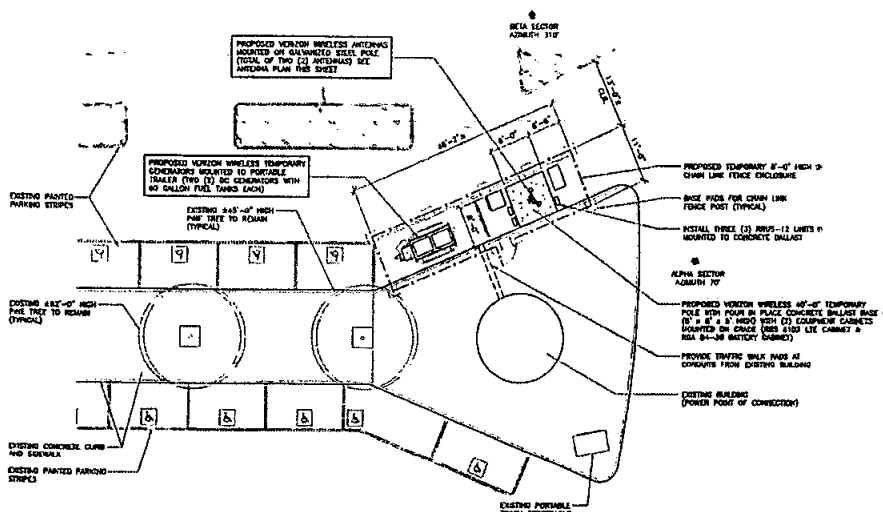
ENLARGED SITE PLAN SITE #1 NORTHEAST SCALE 1" = 10'
