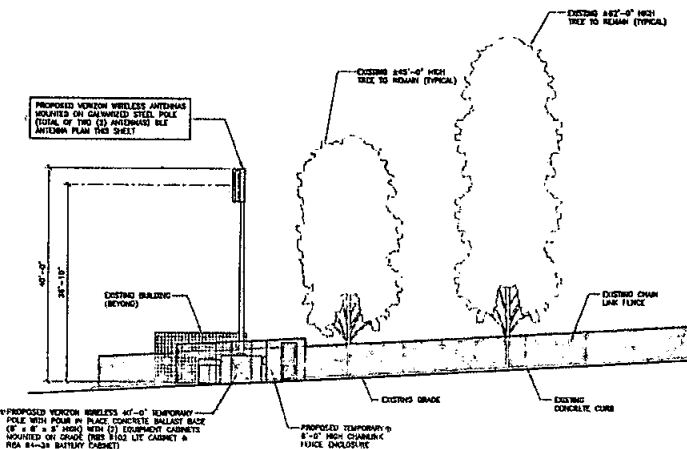
WEST ELEVATION SCALE: 1" = 10'
