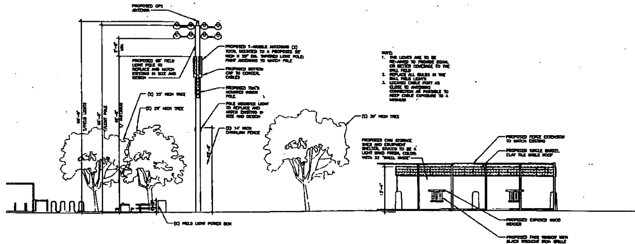
SOUTHWEST ELEVATION 1/8" = 1'-0"
