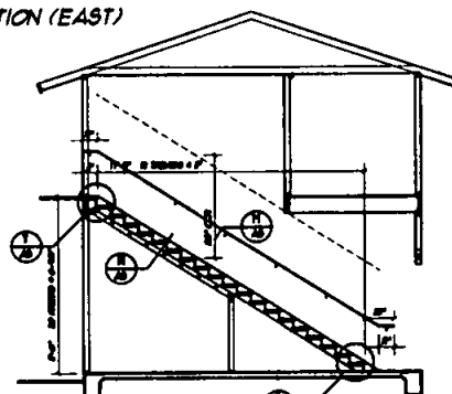
④ ALTERNATE STAIR SECTION
