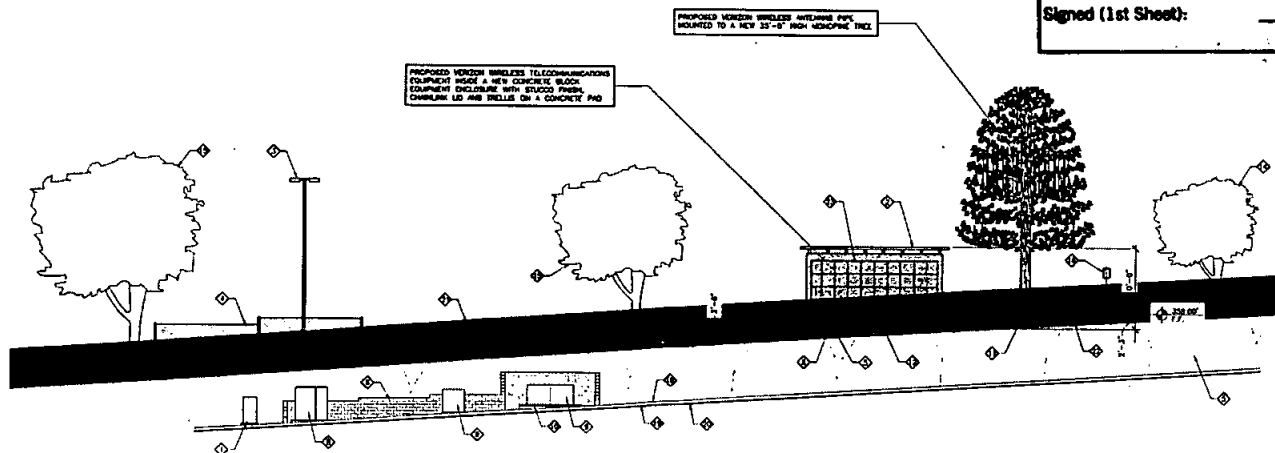
EAST ELEVATION SCALE 1/4" = 1'-0"
