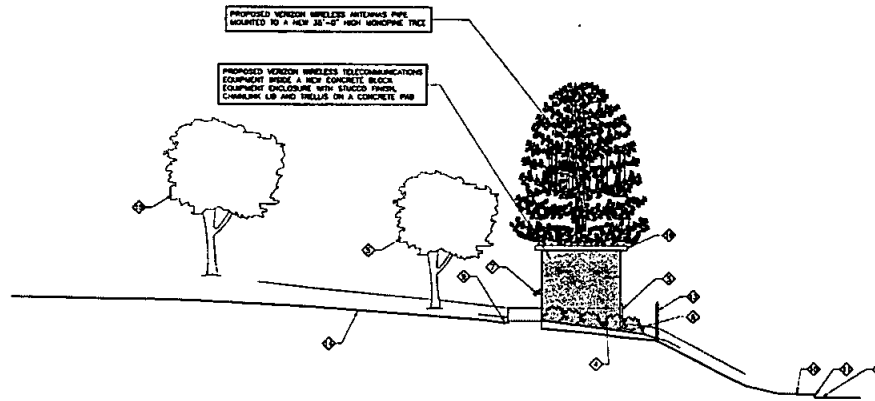
SOUTH ELEVATION SCALE 1/4" = 1'-0"
