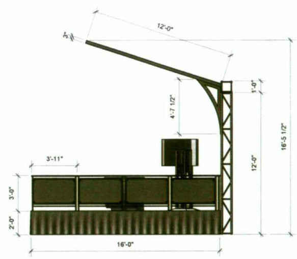
2 FOX PETCO STAGE SIDE Scale: 1/4" = 1'-0"
