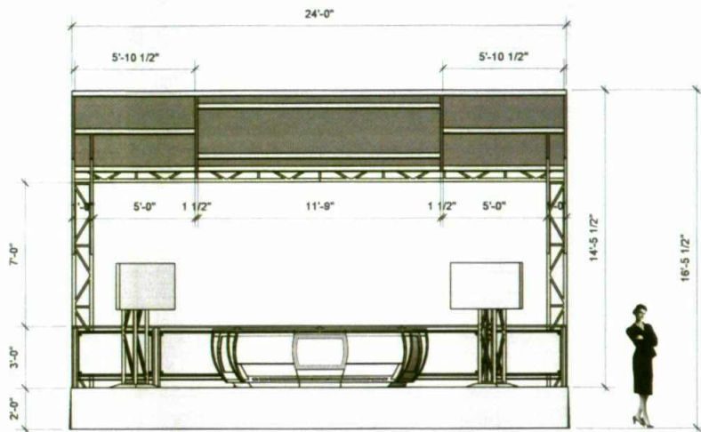
1 FOX PETCO STAGE FRONT Scale: 1/4" = 1'-0"
