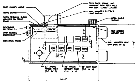
EQUIPMENT PLAN 1/4"=1'-0"
