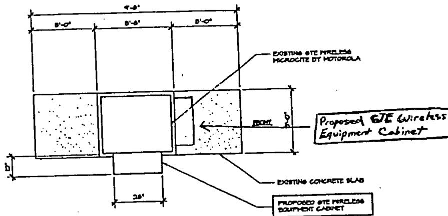
ENLARGED SITE PLAN SCALE: 1/8" = 1'-0"
