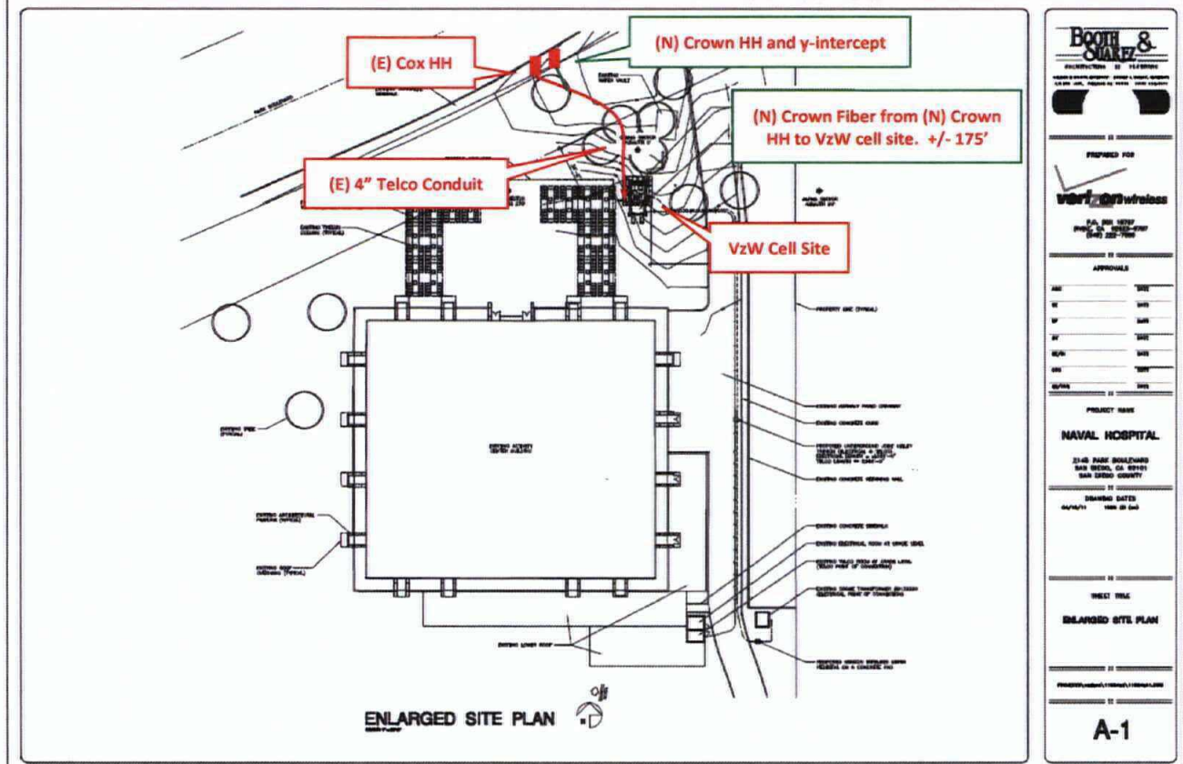
Overall view of fiber path (locations and distances are approximate)
