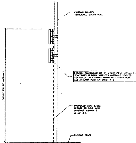
TYPICAL POLE PROFILE SCALE 1/4" = 1'-0"
