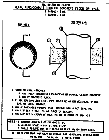
HILTI FIRESTOP DETAIL
