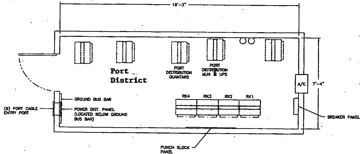
EQUIPMENT ROOM EQUIPMENT LAYOUT - PLAN VIEW
